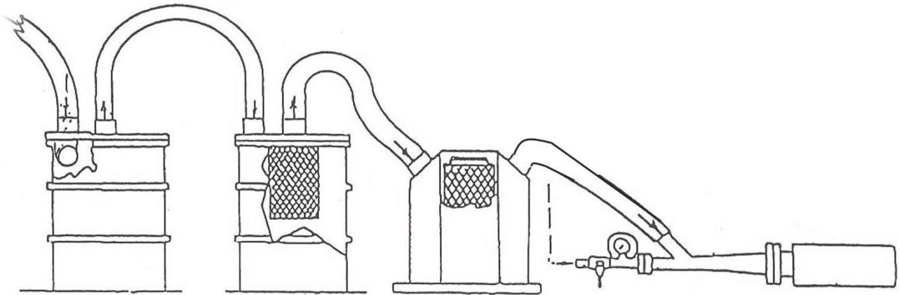
Figure #4 CBS Kit "C" – Single Pump w/ H.E.P.A.
